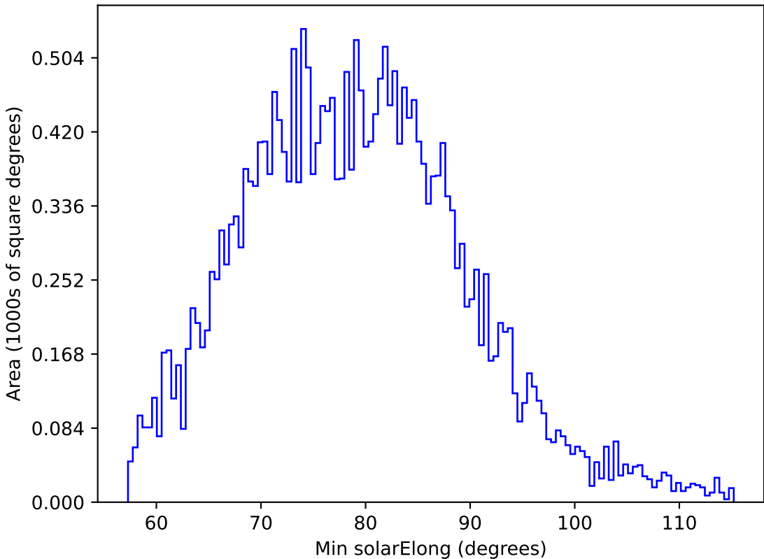
ddf_loaded_half_fl2_v3.4_10yrs All sky g band: Min solarElong
