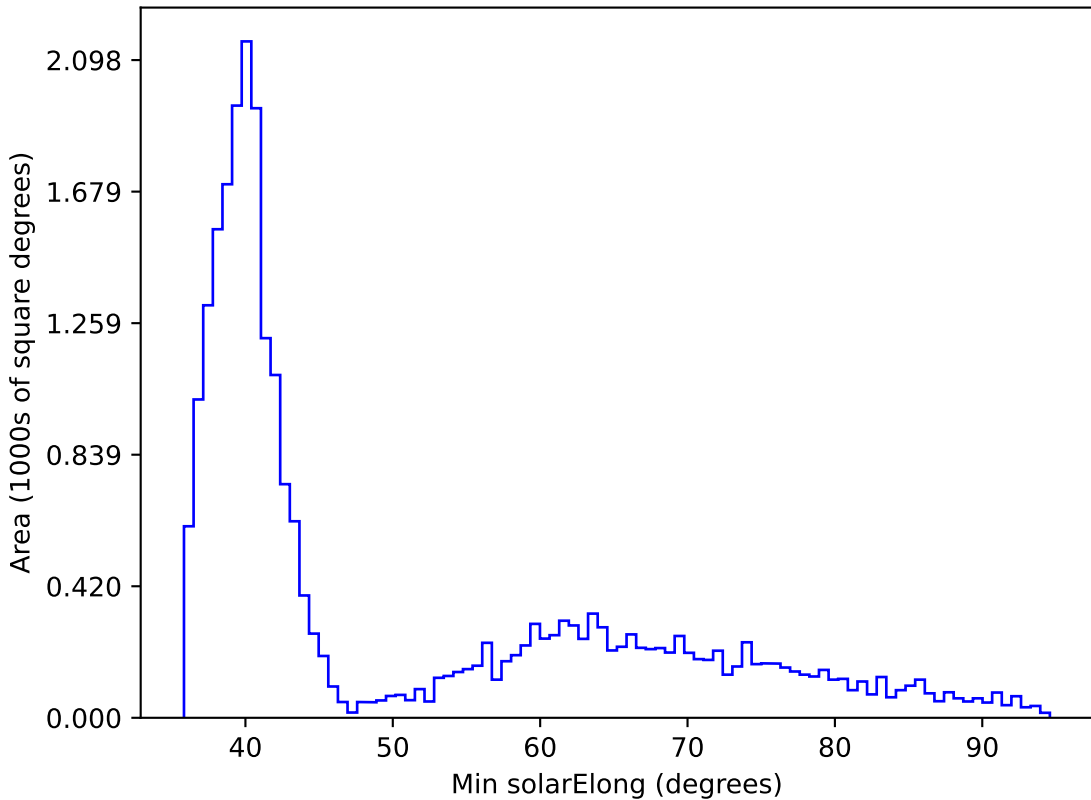
ddf_loaded_half_fl2_v3.4_10yrs All sky all bands: Min solarElong
