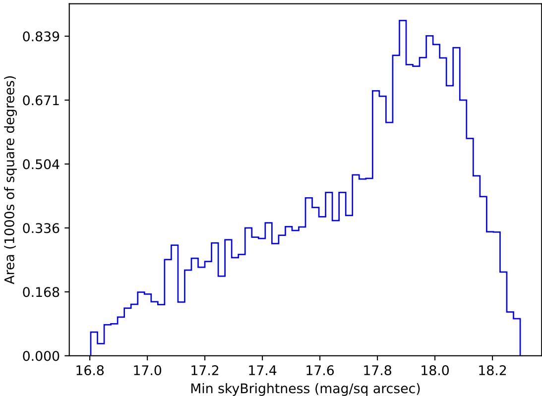
ddf_loaded_half_fl2_v3.4_10yrs Yr 1 y band: Min skyBrightness
