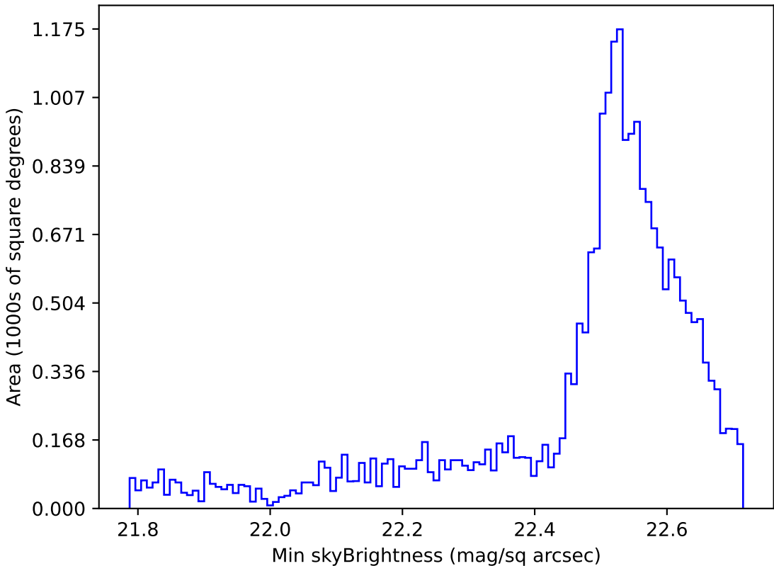
ddf_loaded_half_fl2_v3.4_10yrs Yr 1 u band: Min skyBrightness
