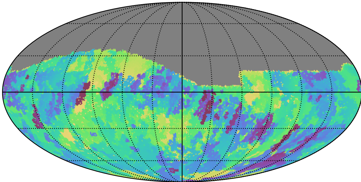
ddf_loaded_half_fl2_v3.4_10yrs Yr 1 r band: Min skyBrightness
