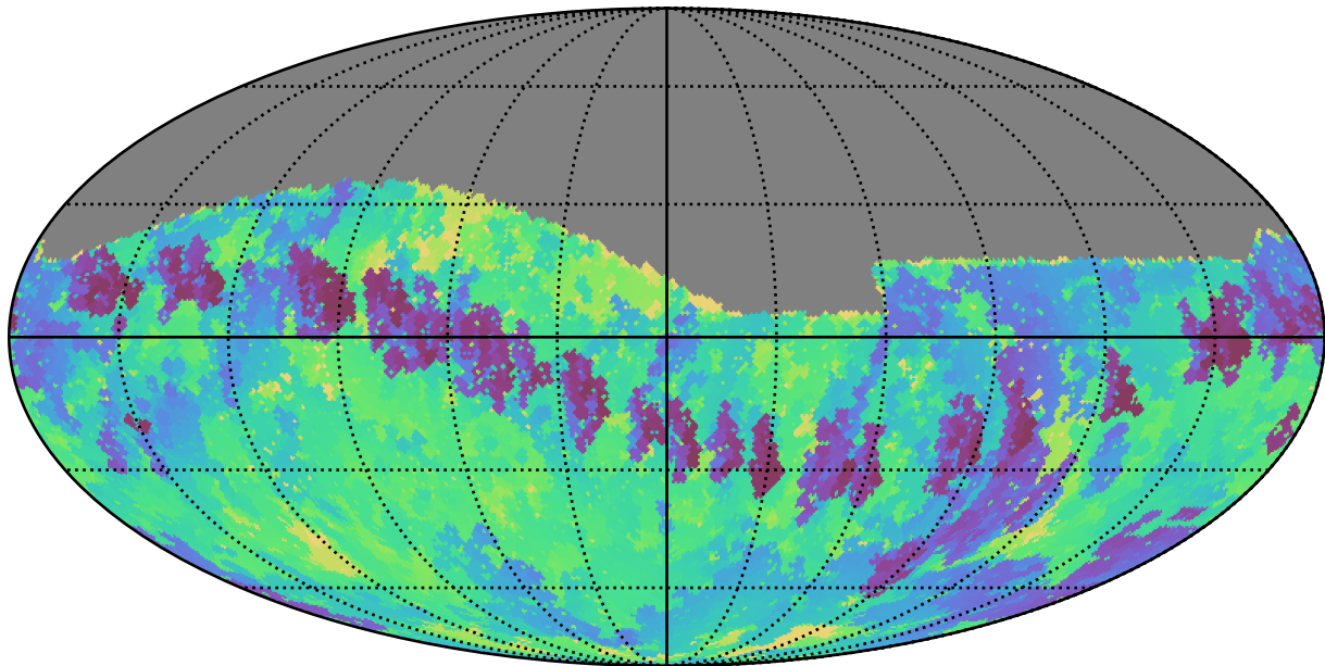
ddf_loaded_half_fl2_v3.4_10yrs Yr 1 i band: Min skyBrightness
