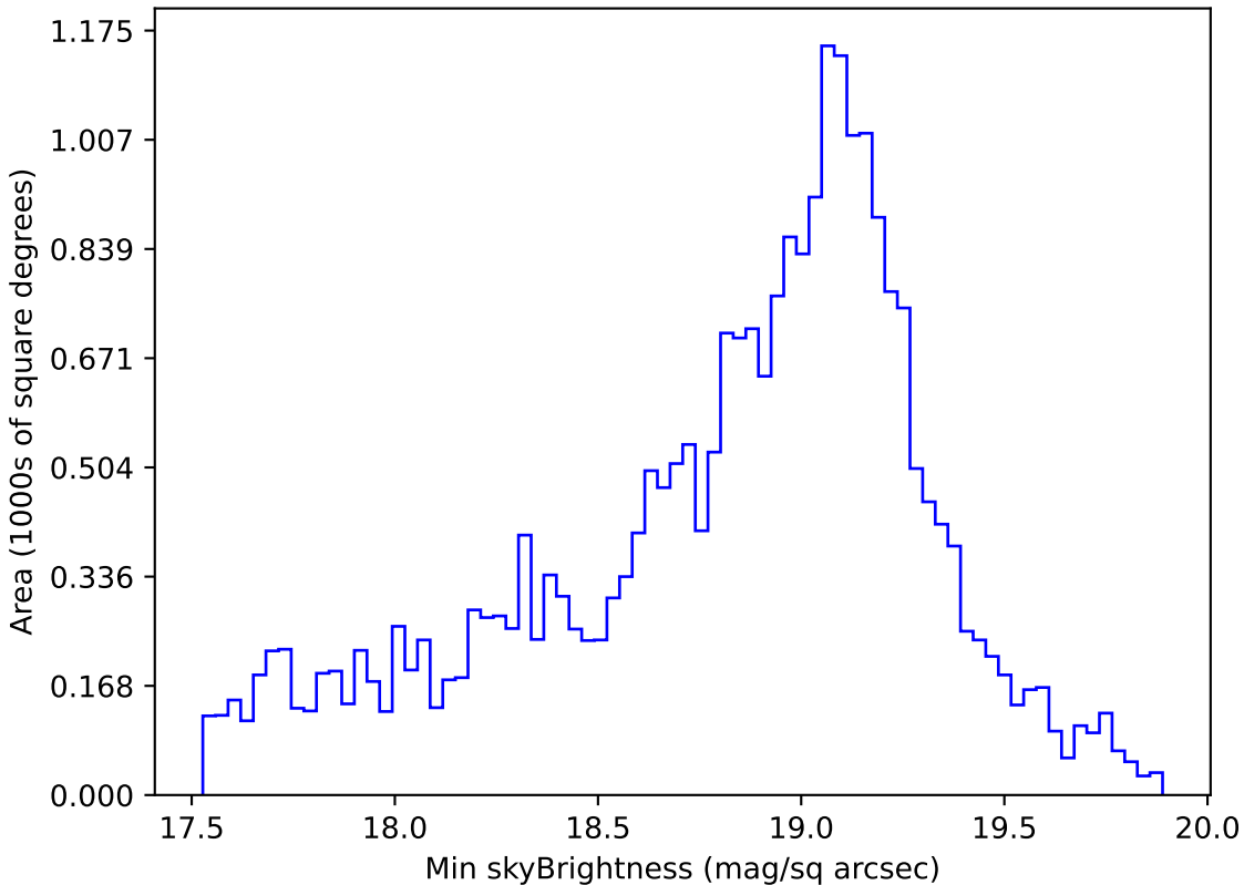
ddf_loaded_half_fl2_v3.4_10yrs Yr 1 i band: Min skyBrightness
