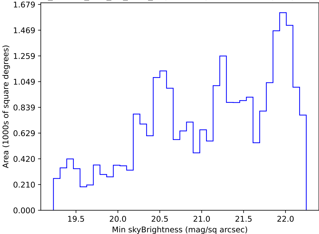
ddf_loaded_half_fl2_v3.4_10yrs Yr 1 g band: Min skyBrightness
