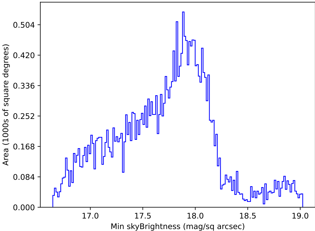
ddf_loaded_half_fl2_v3.4_10yrs Yr 1 all bands: Min skyBrightness
