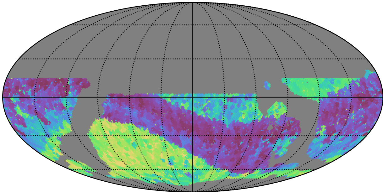
ddf_loaded_half_fl2_v3.4_10yrs WFD z band: Min skyBrightness
