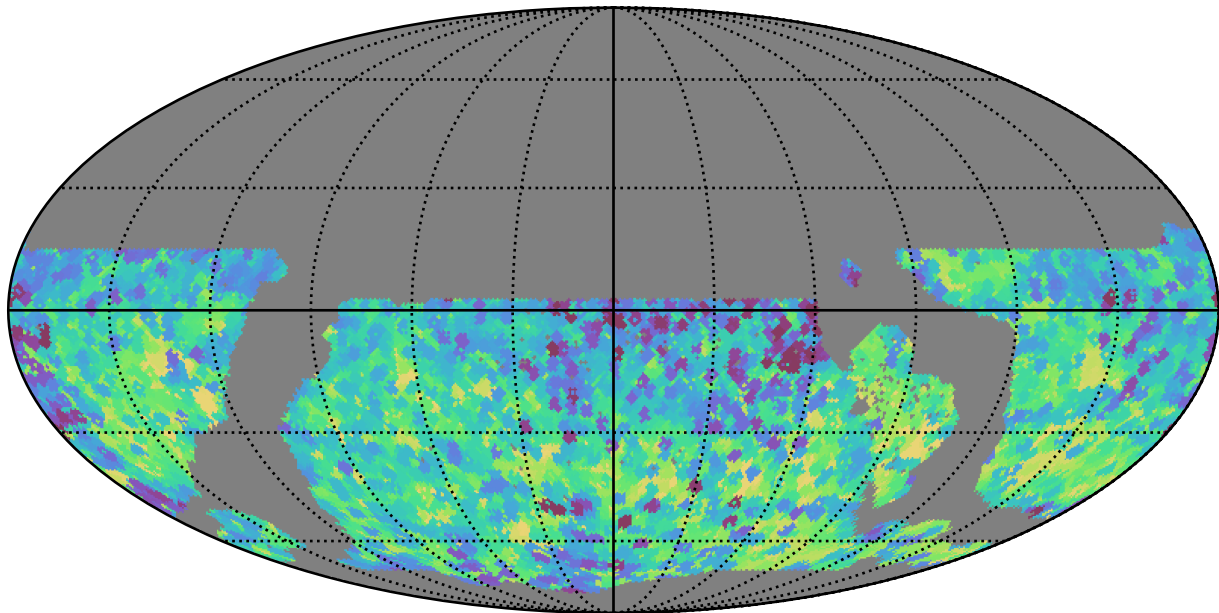
ddf_loaded_half_fl2_v3.4_10yrs WFD y band: Min skyBrightness
