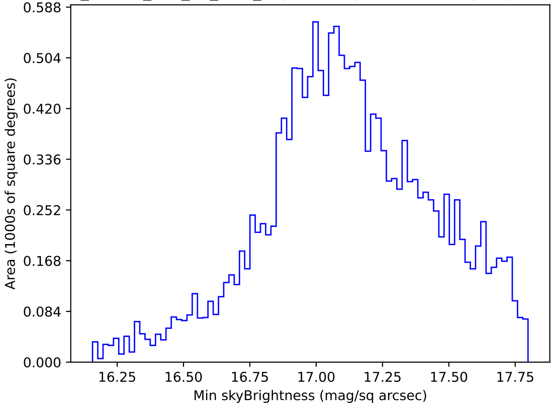
ddf_loaded_half_fl2_v3.4_10yrs WFD y band: Min skyBrightness
