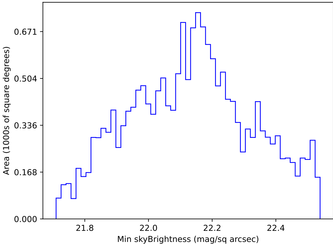
ddf_loaded_half_fl2_v3.4_10yrs WFD u band: Min skyBrightness
