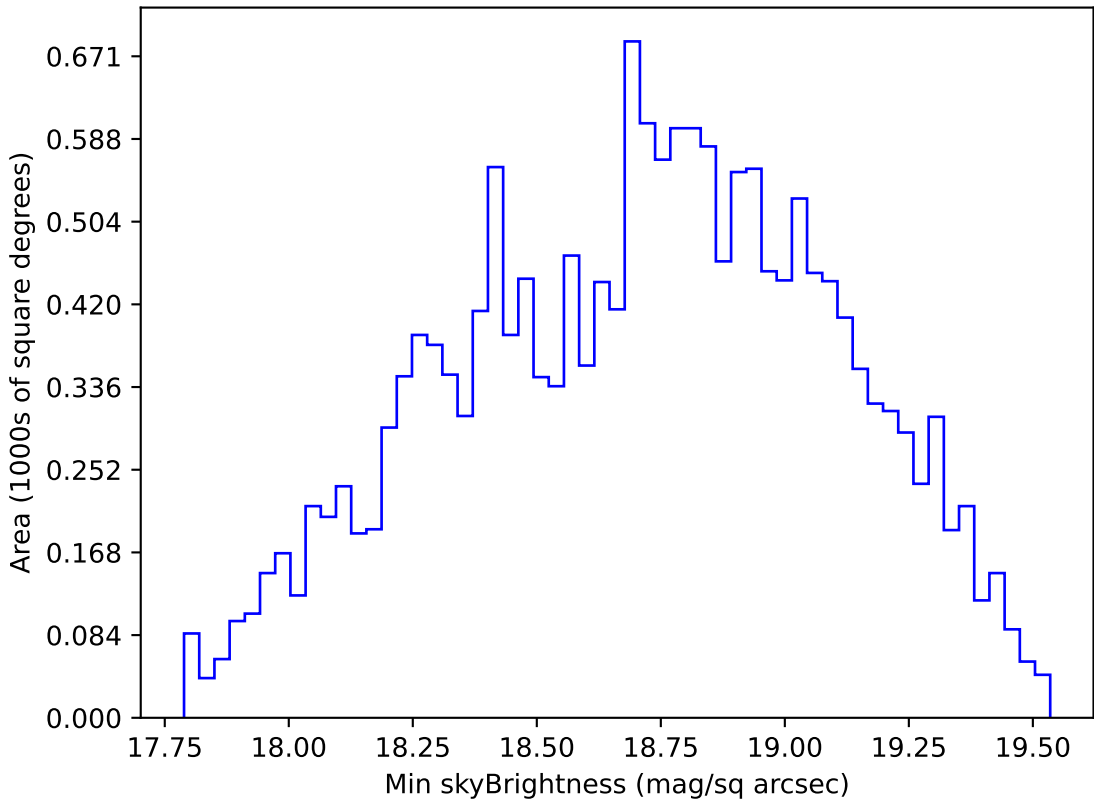
ddf_loaded_half_fl2_v3.4_10yrs WFD r band: Min skyBrightness
