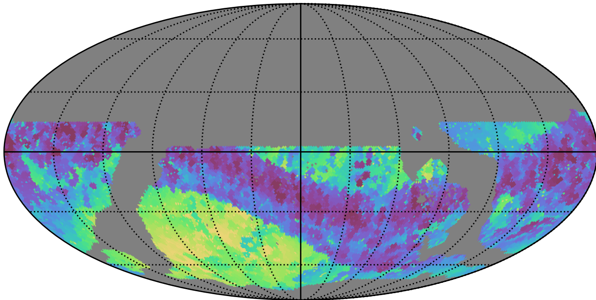
ddf_loaded_half_fl2_v3.4_10yrs WFD i band: Min skyBrightness
