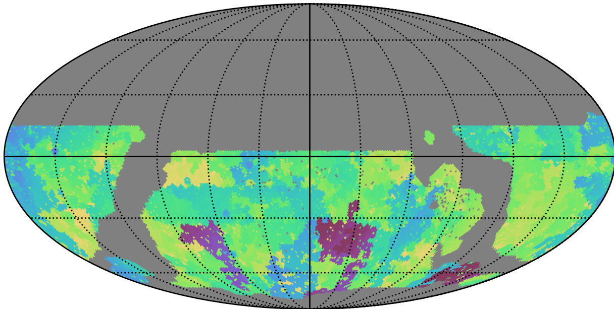
ddf_loaded_half_fl2_v3.4_10yrs WFD g band: Min skyBrightness
