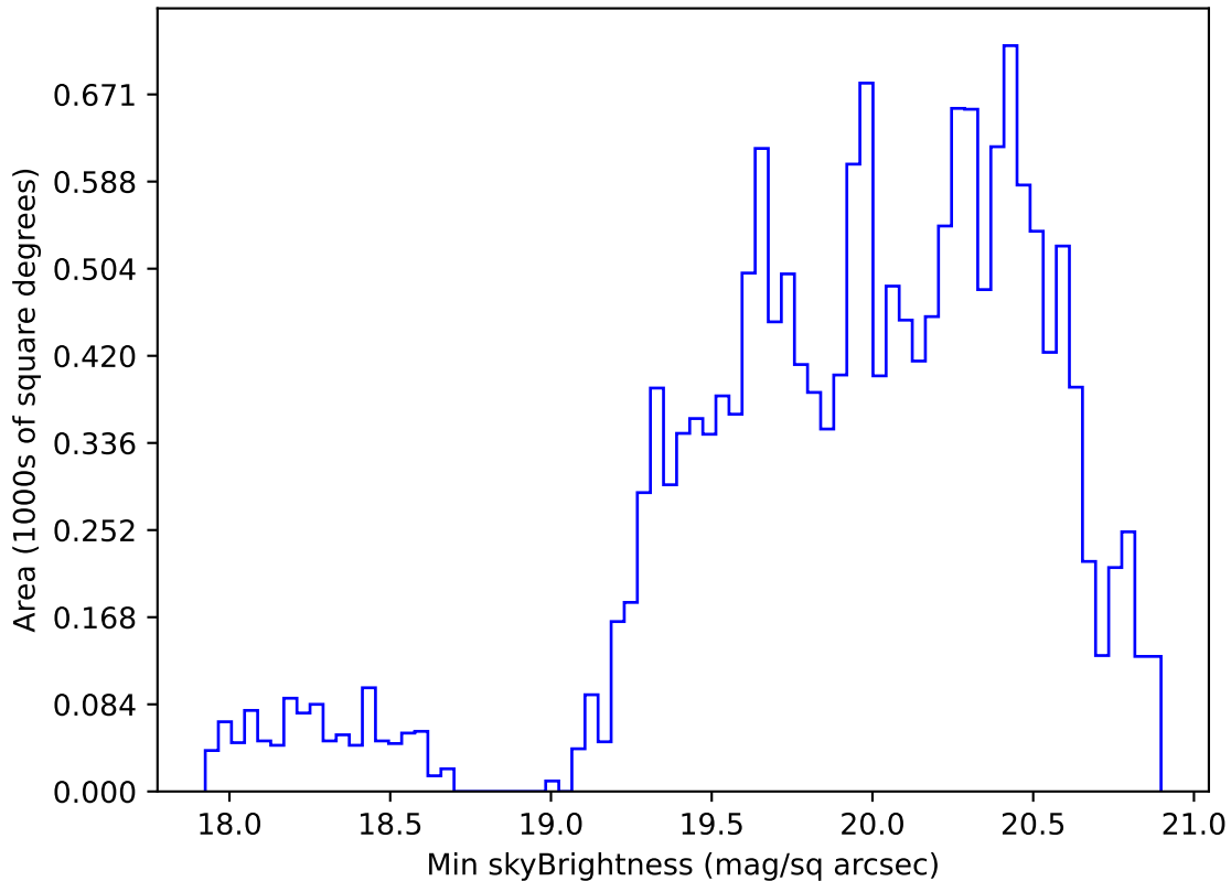
ddf_loaded_half_fl2_v3.4_10yrs WFD g band: Min skyBrightness
