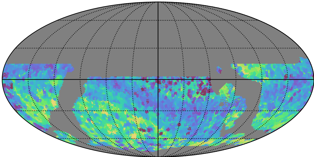
ddf_loaded_half_fl2_v3.4_10yrs WFD all bands: Min skyBrightness
