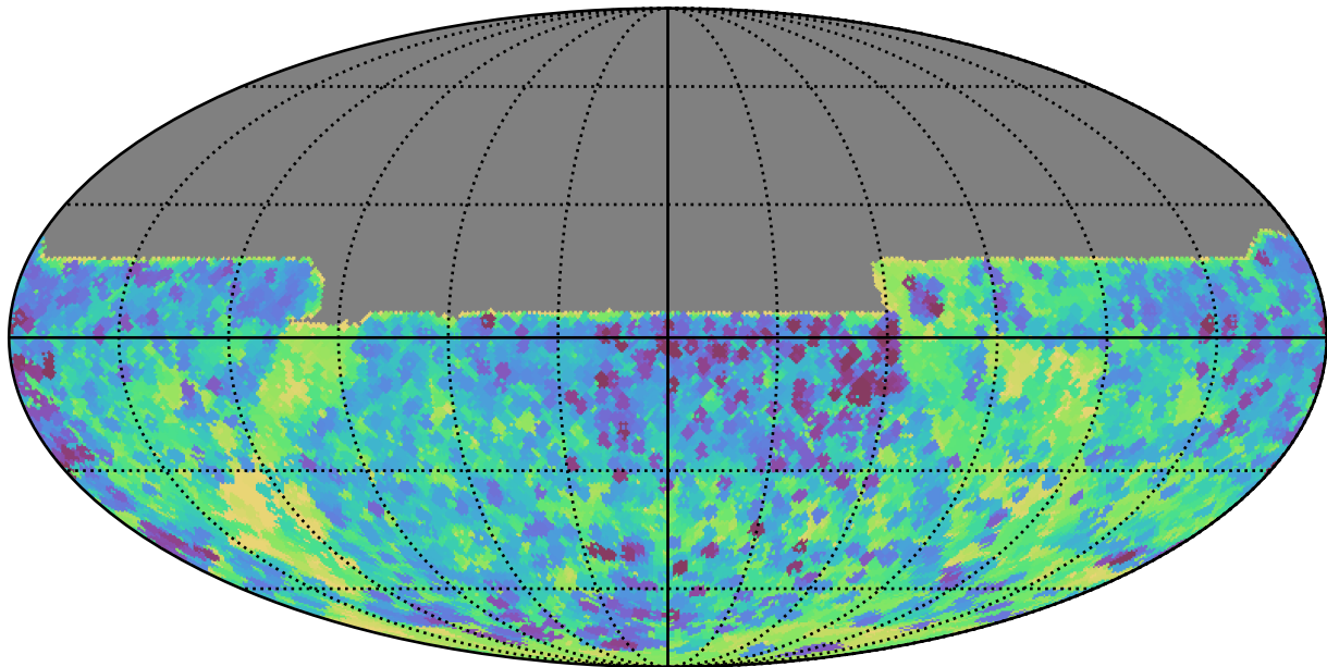
ddf_loaded_half_fl2_v3.4_10yrs All sky y band: Min skyBrightness
