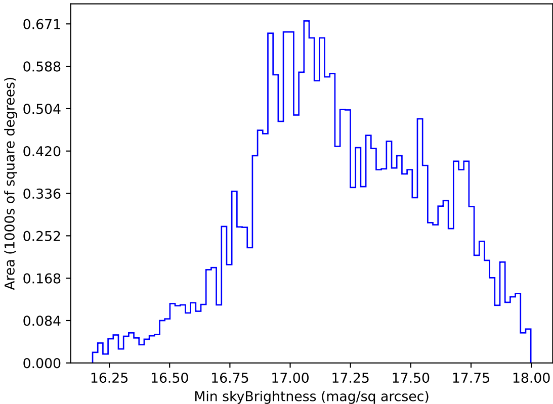
ddf_loaded_half_fl2_v3.4_10yrs All sky y band: Min skyBrightness
