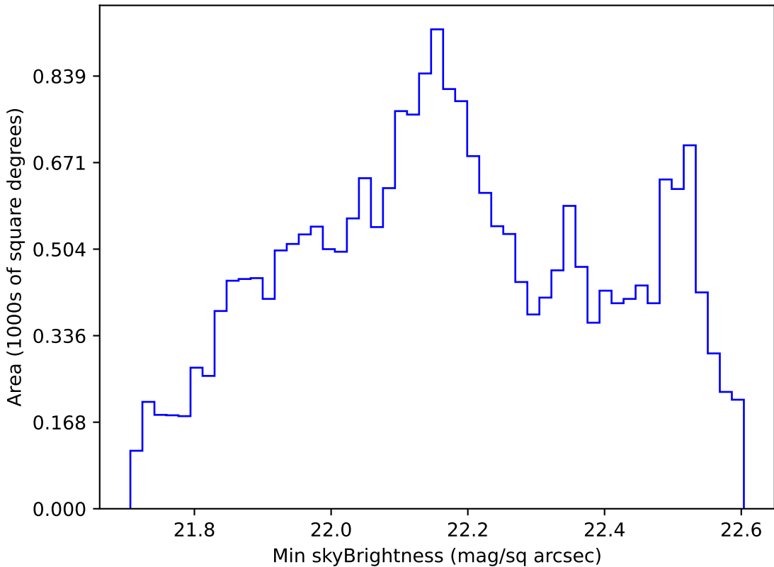
ddf_loaded_half_fl2_v3.4_10yrs All sky u band: Min skyBrightness
