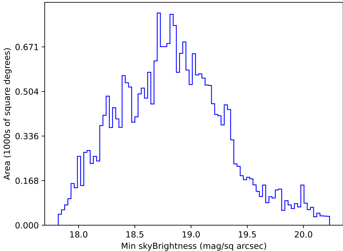
ddf_loaded_half_fl2_v3.4_10yrs All sky r band: Min skyBrightness
