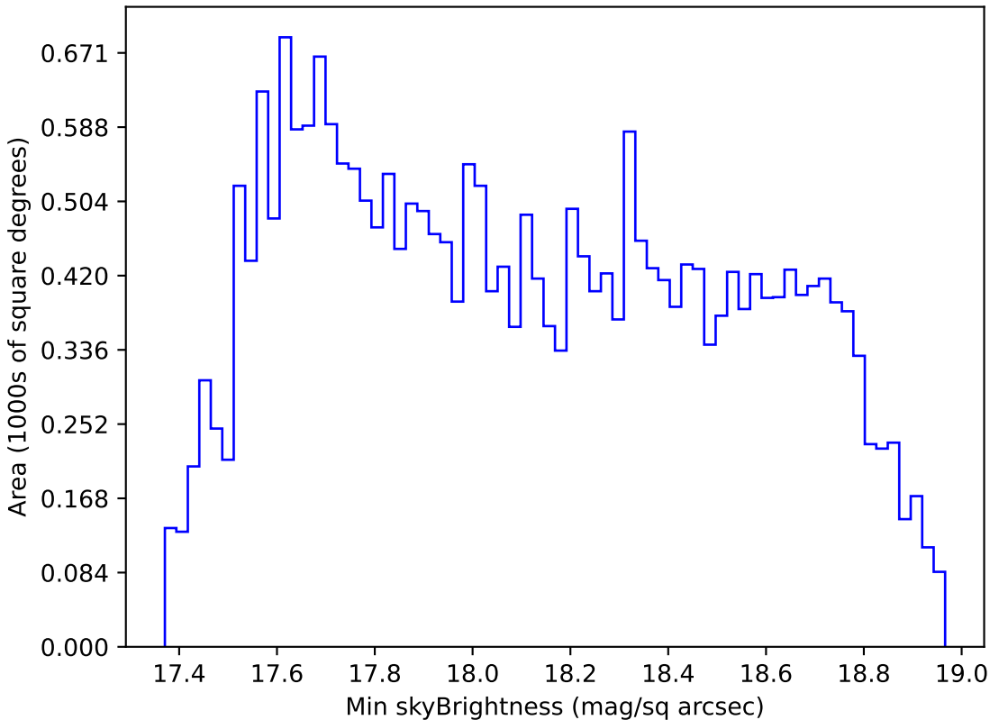
ddf_loaded_half_fl2_v3.4_10yrs All sky i band: Min skyBrightness
