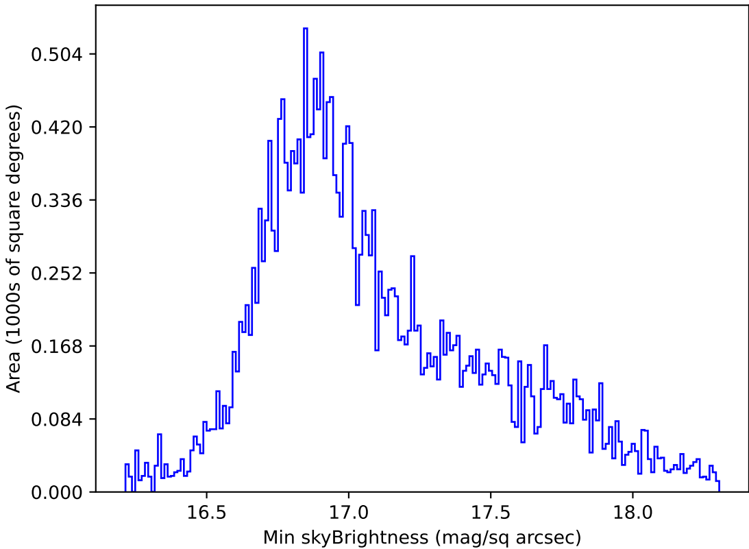
ddf_loaded_half_fl2_v3.4_10yrs All sky all bands: Min skyBrightness
