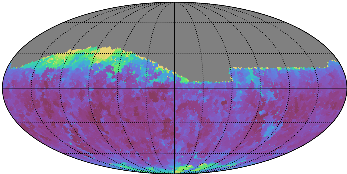
ddf_loaded_half_fl2_v3.4_10yrs Yr 1 r band: Min seeingGeom
