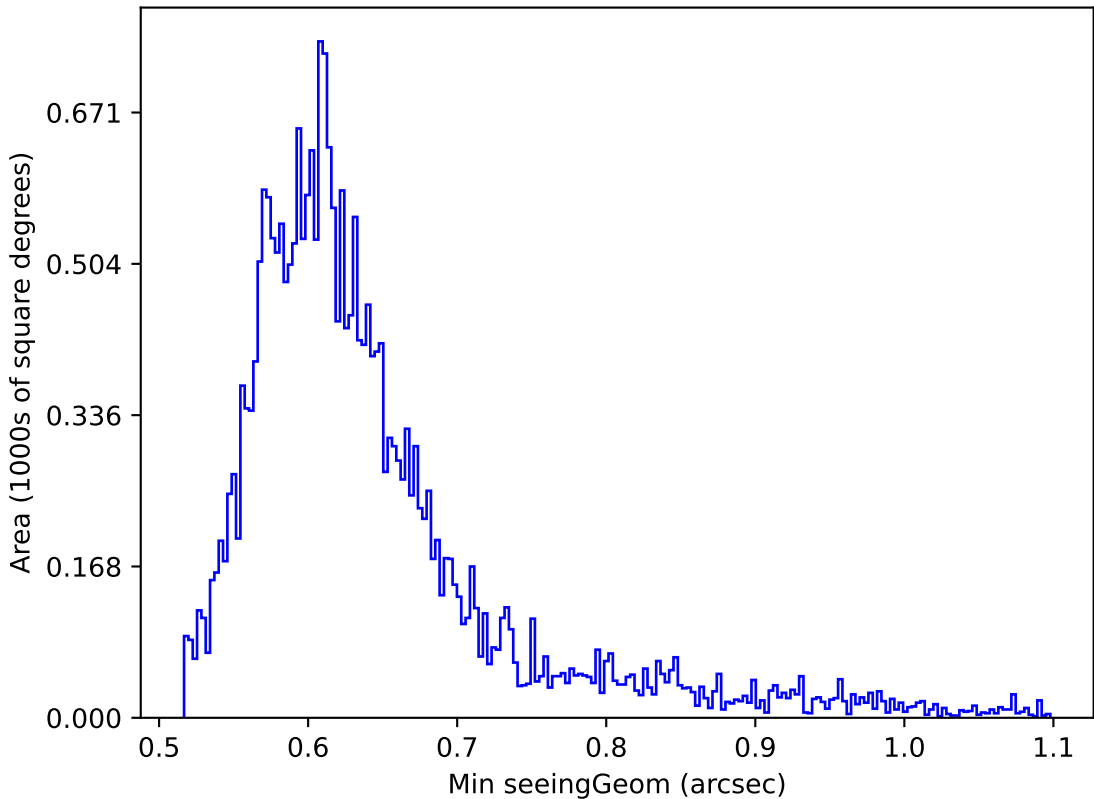
ddf_loaded_half_fl2_v3.4_10yrs Yr 1 r band: Min seeingGeom
