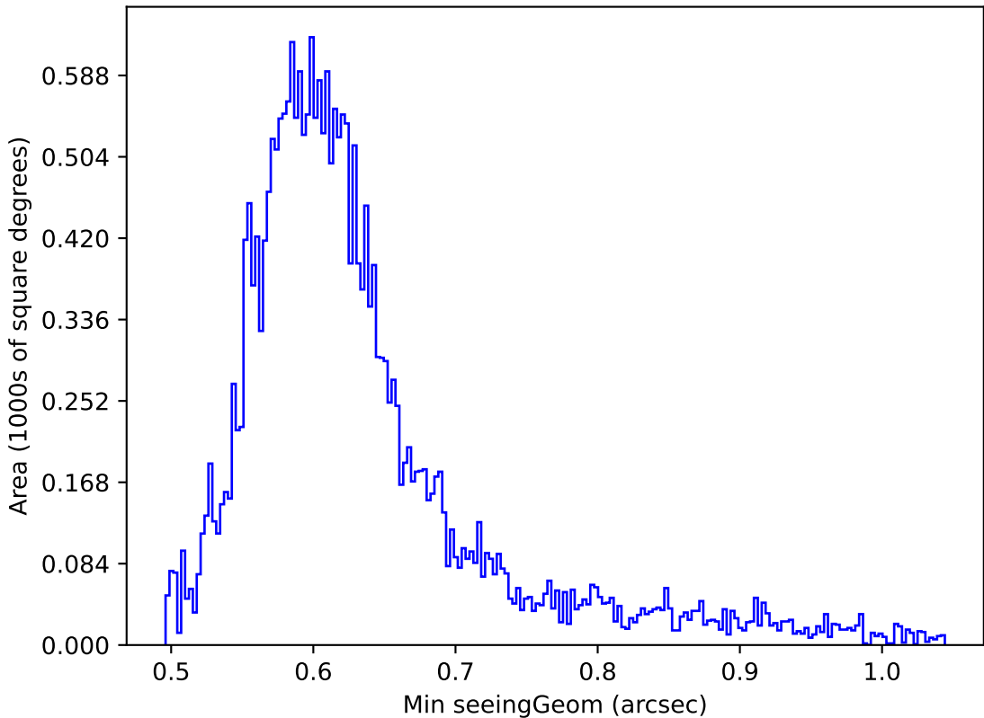
ddf_loaded_half_fl2_v3.4_10yrs Yr 1 i band: Min seeingGeom
