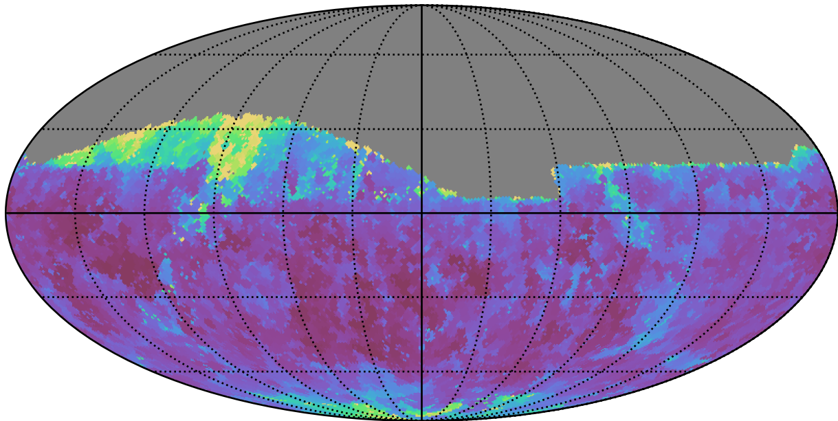
ddf_loaded_half_fl2_v3.4_10yrs Yr 1 z band: Min seeingEff
