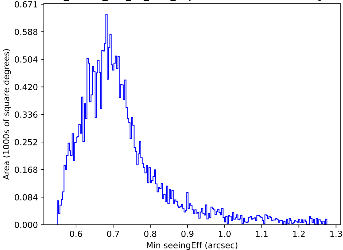
ddf_loaded_half_fl2_v3.4_10yrs Yr 1 z band: Min seeingEff
