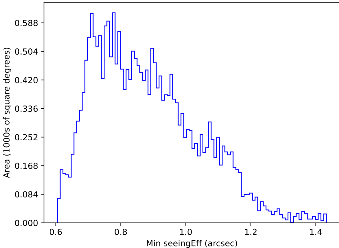
ddf_loaded_half_fl2_v3.4_10yrs Yr 1 u band: Min seeingEff
