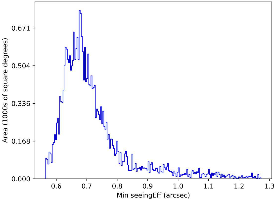
ddf_loaded_half_fl2_v3.4_10yrs Yr 1 r band: Min seeingEff
