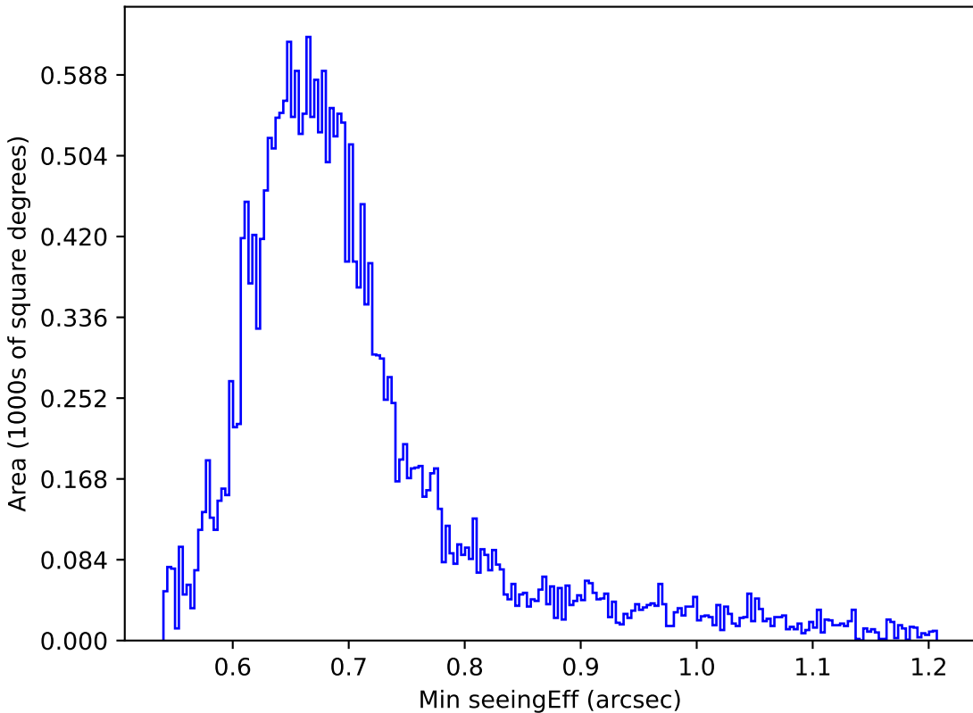
ddf_loaded_half_f12_v3.4_10yrs Yr 1 i band: Min seeingEff
