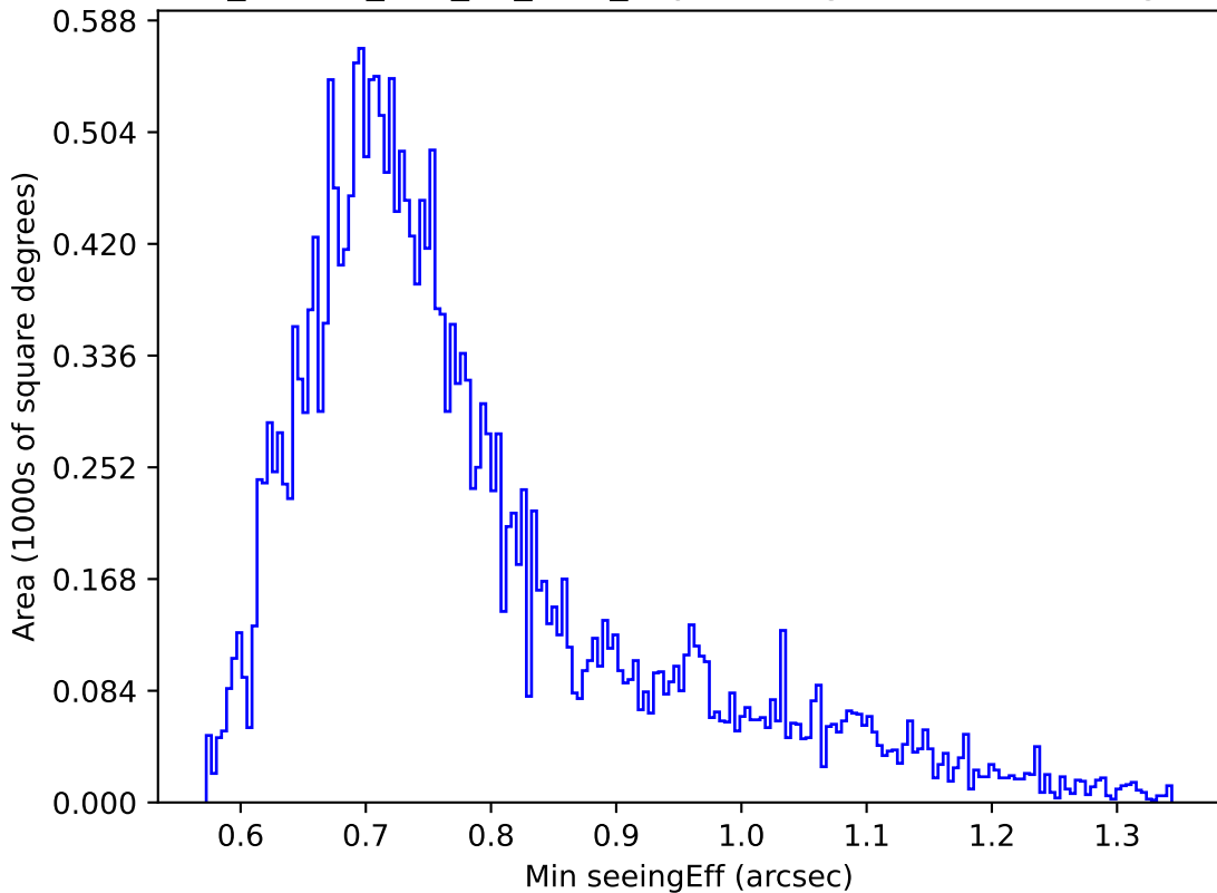
ddf_loaded_half_fl2_v3.4_10yrs Yr 1 g band: Min seeingEff
