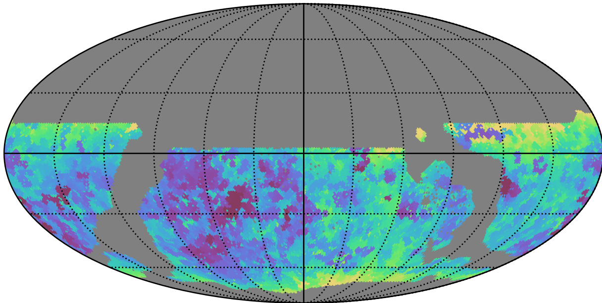
ddf_loaded_half_fl2_v3.4_10yrs WFD r band: Min seeingEff
