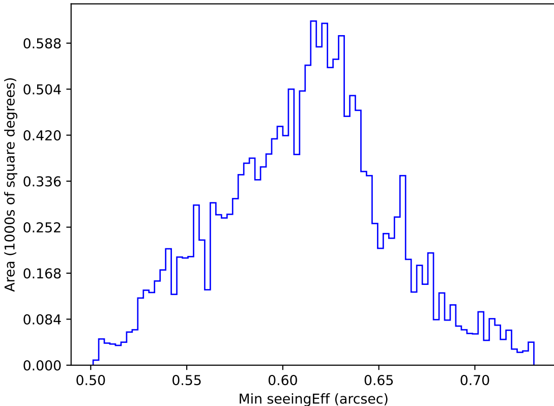
ddf_loaded_half_fl2_v3.4_10yrs WFD r band: Min seeingEff
