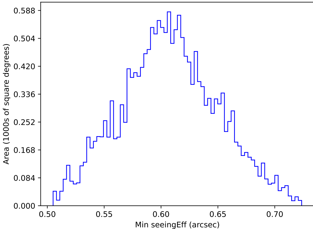
ddf_loaded_half_fl2_v3.4_10yrs WFD i band: Min seeingEff
