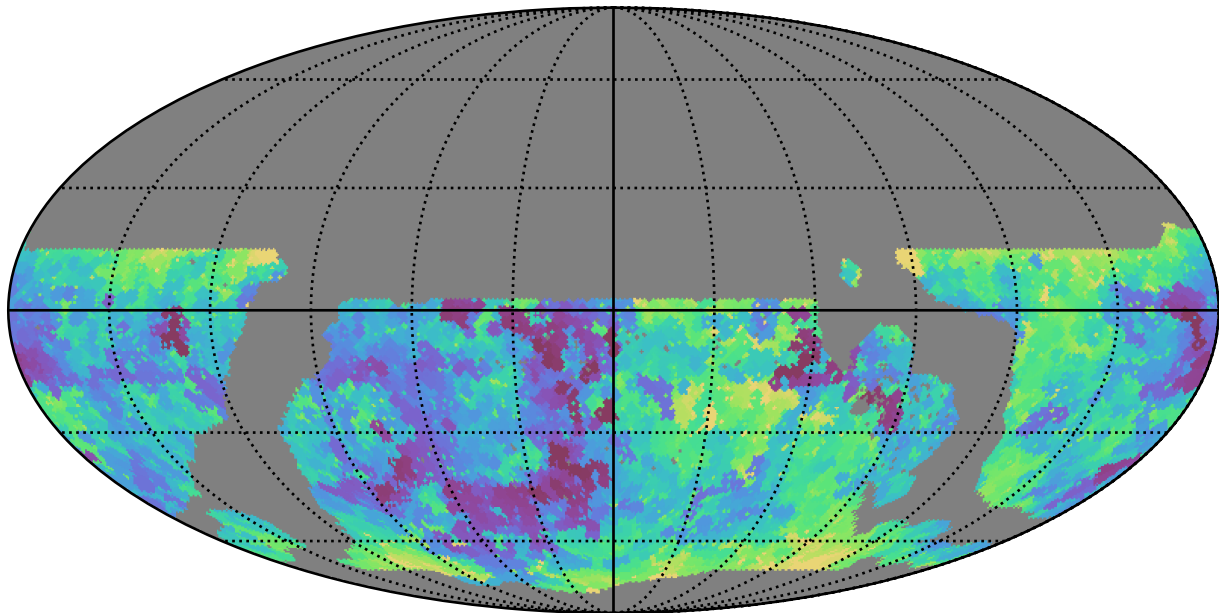
ddf_loaded_half_fl2_v3.4_10yrs WFD g band: Min seeingEff
