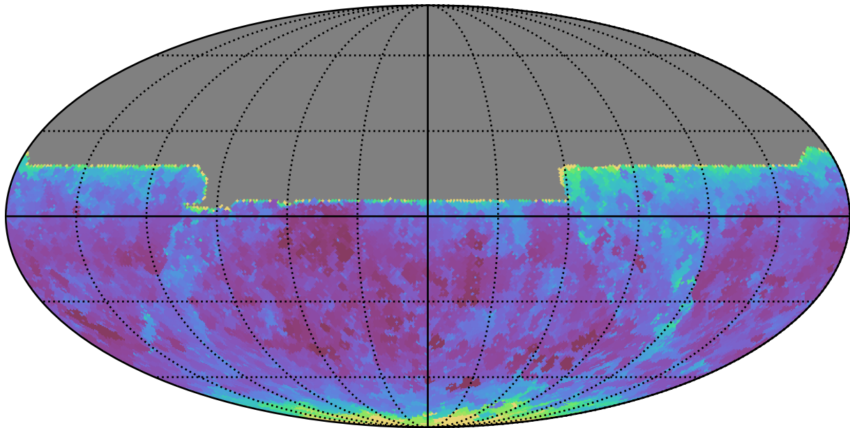
ddf_loaded_half_fl2_v3.4_10yrs All sky y band: Min seeingEff
