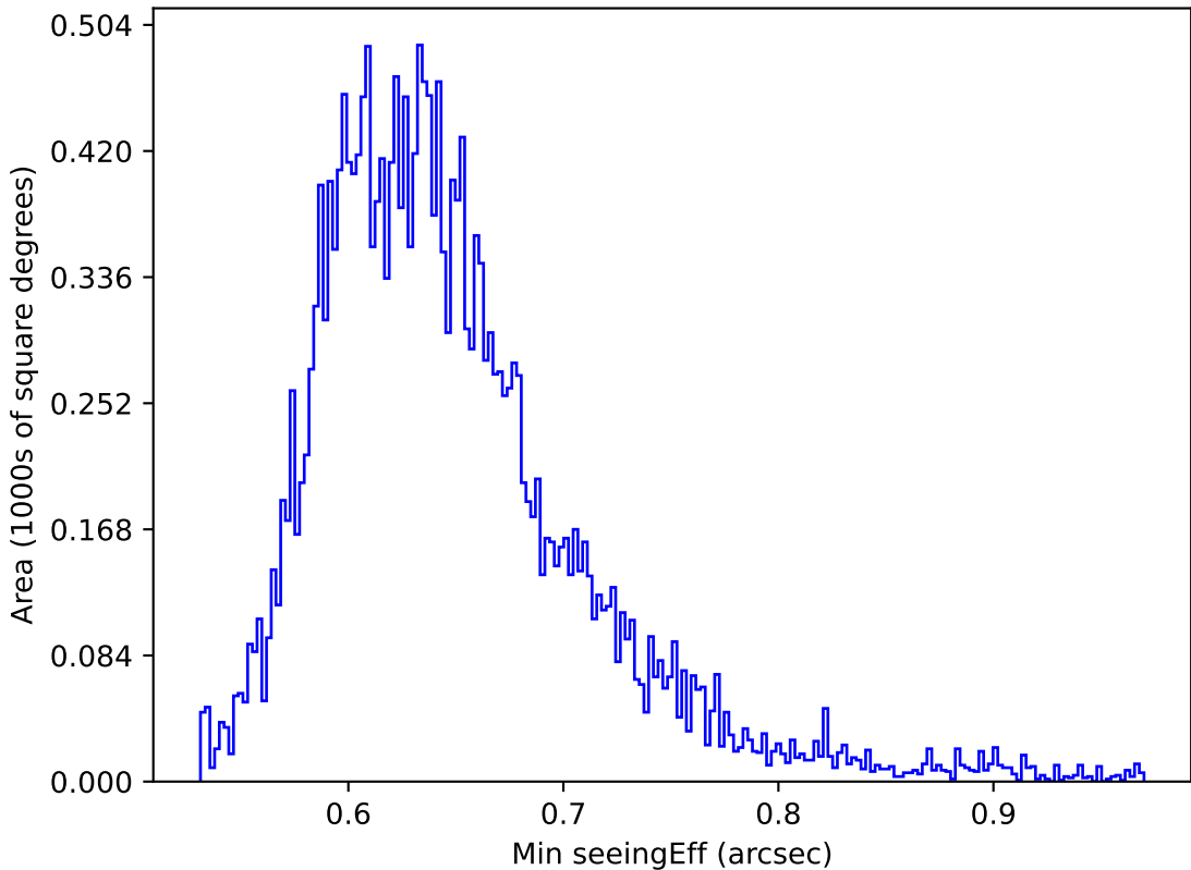
ddf_loaded_half_fl2_v3.4_10yrs All sky y band: Min seeingEff
