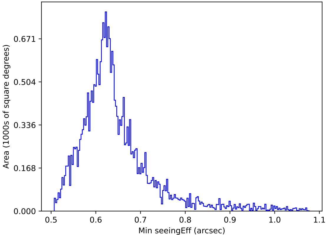
ddf_loaded_half_fl2_v3.4_10yrs All sky r band: Min seeingEff
