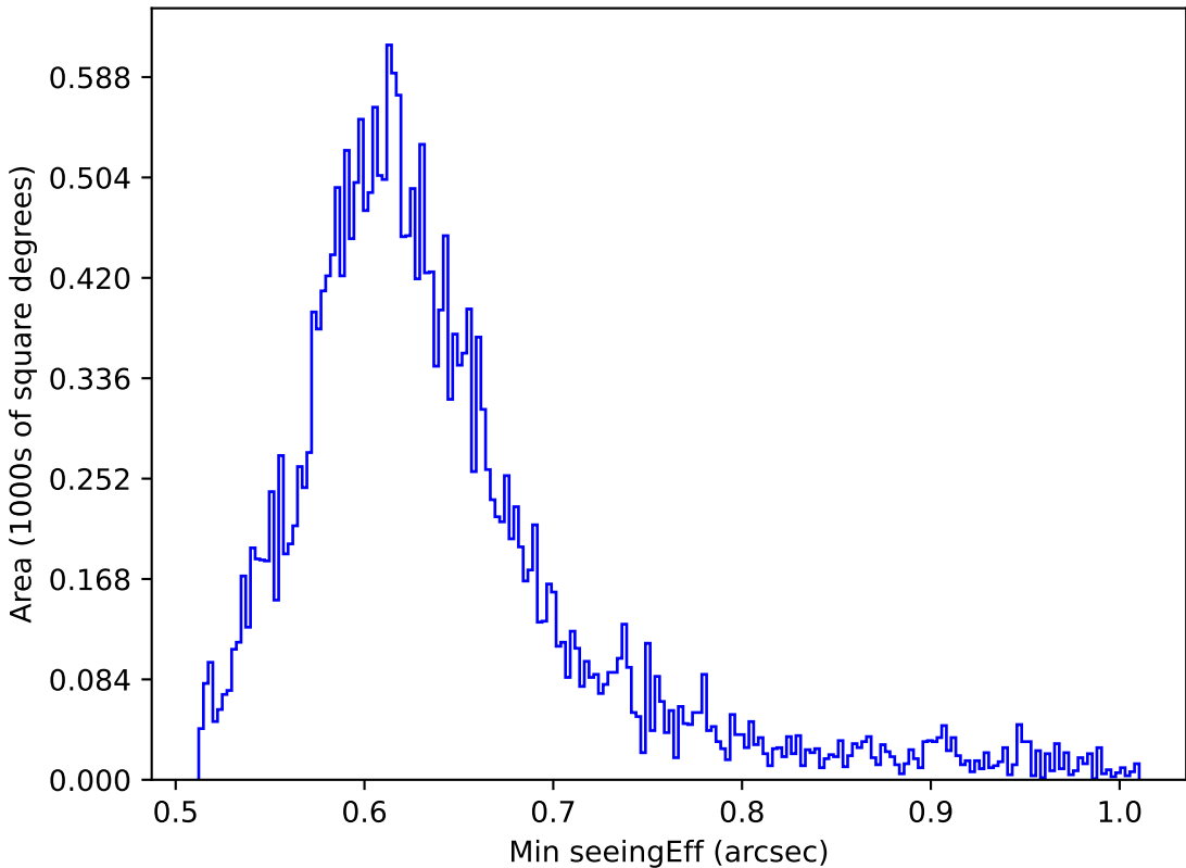
ddf_loaded_half_fl2_v3.4_10yrs All sky i band: Min seeingEff
