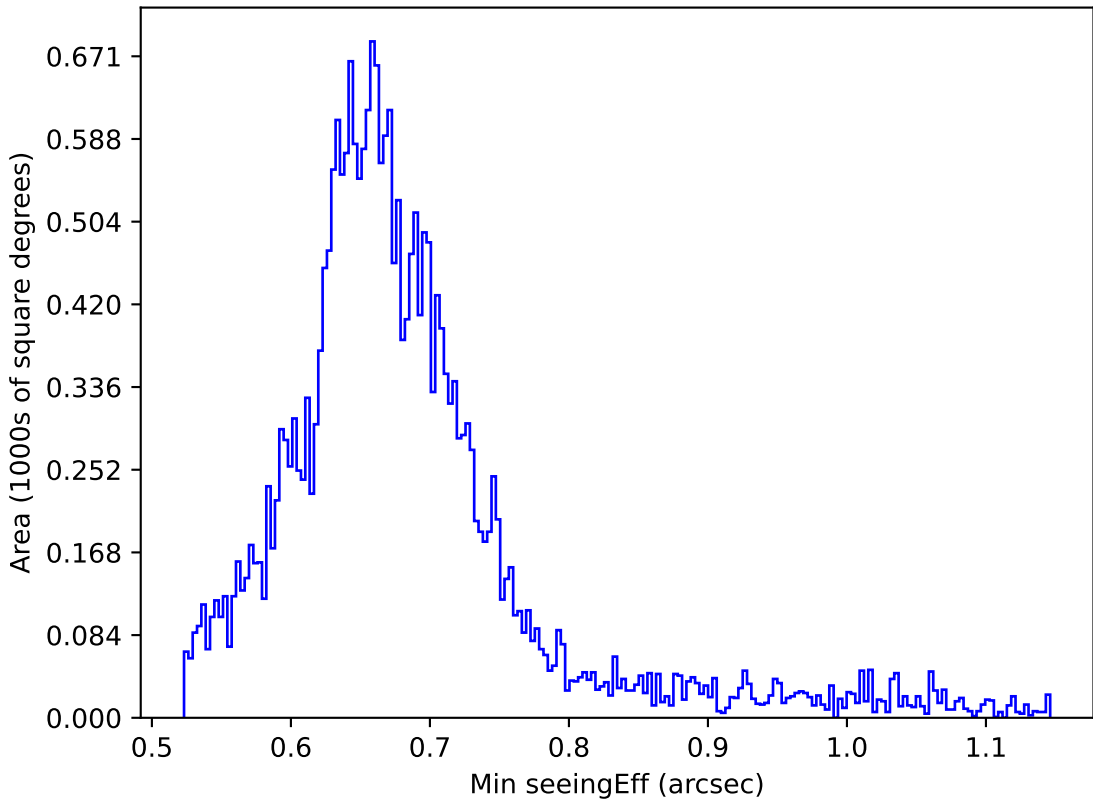
ddf_loaded_half_fl2_v3.4_10yrs All sky g band: Min seeingEff
