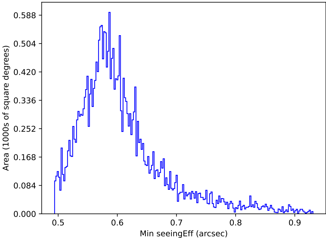
ddf_loaded_half_fl2_v3.4_10yrs All sky all bands: Min seeingEff
