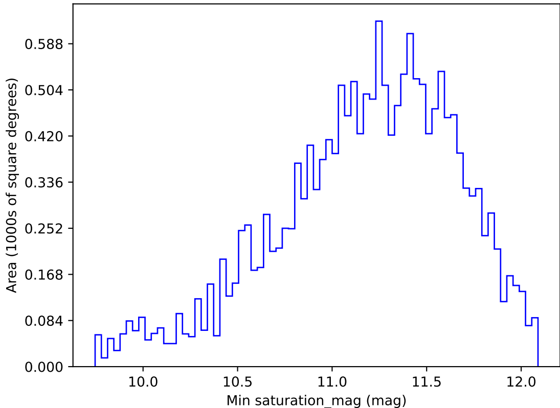
ddf_loaded_half_fl2_v3.4_10yrs WFD y band: Min saturation_mag
