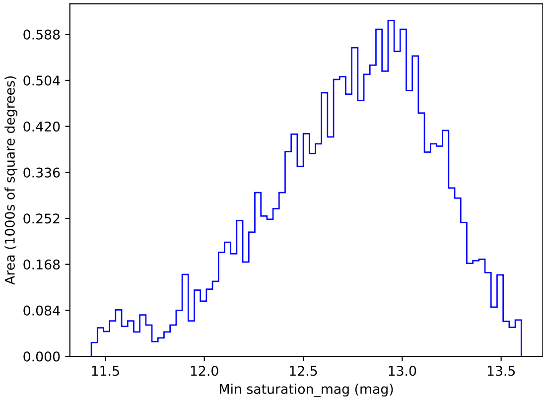
ddf_loaded_half_fl2_v3.4_10yrs WFD g band: Min saturation_mag
