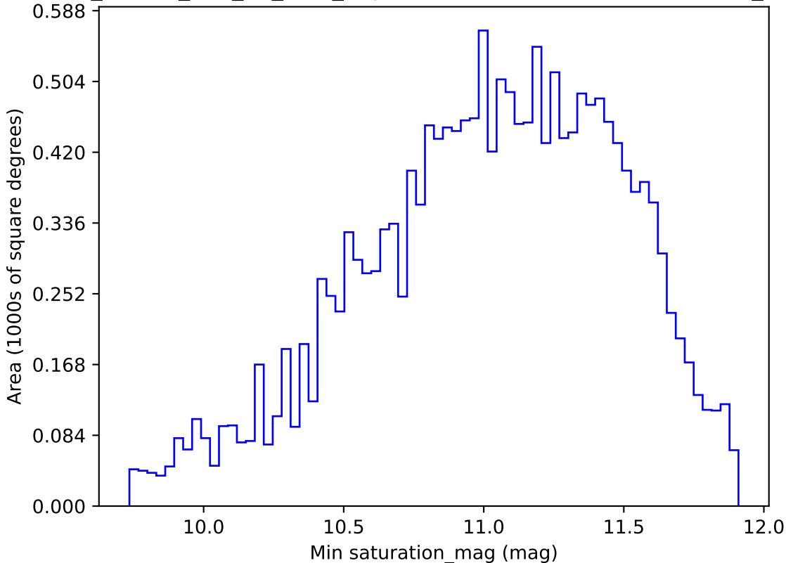
ddf_loaded_half_fl2_v3.4_10yrs WFD all bands: Min saturation_mag
