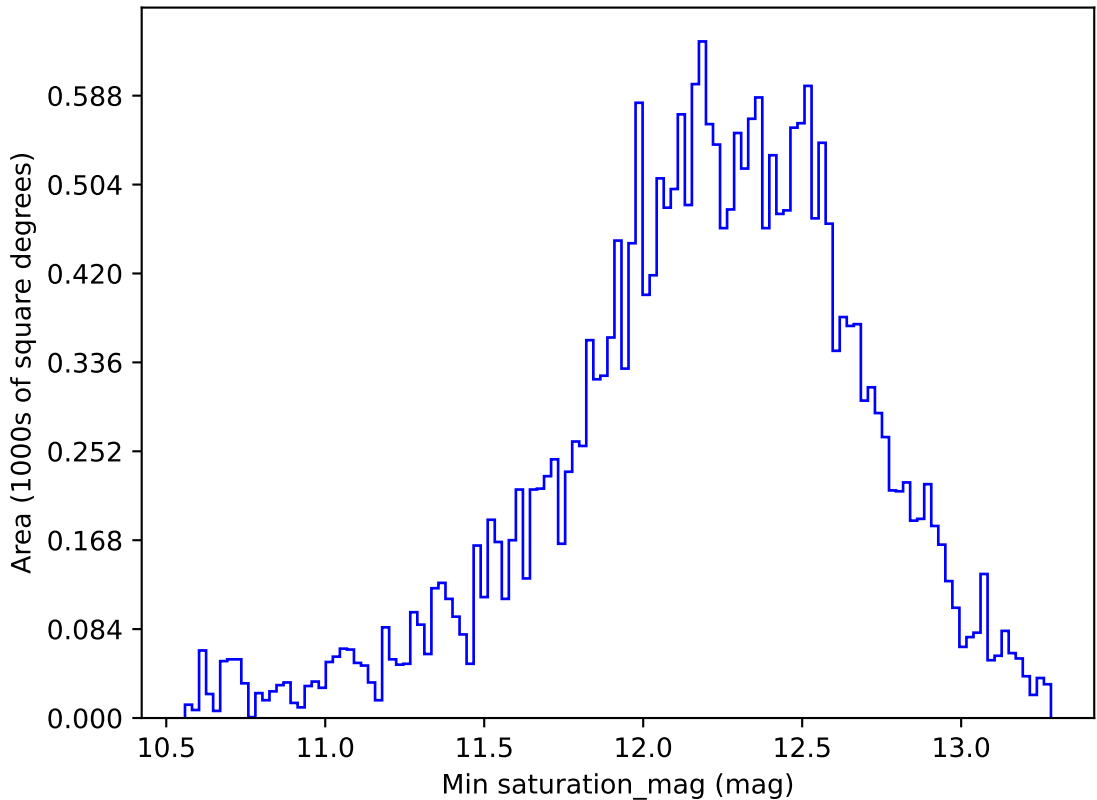
ddf_loaded_half_fl2_v3.4_10yrs All sky z band: Min saturation_mag
