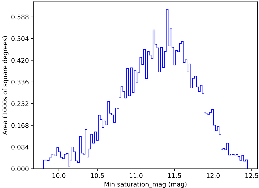
ddf_loaded_half_fl2_v3.4_10yrs All sky y band: Min saturation_mag
