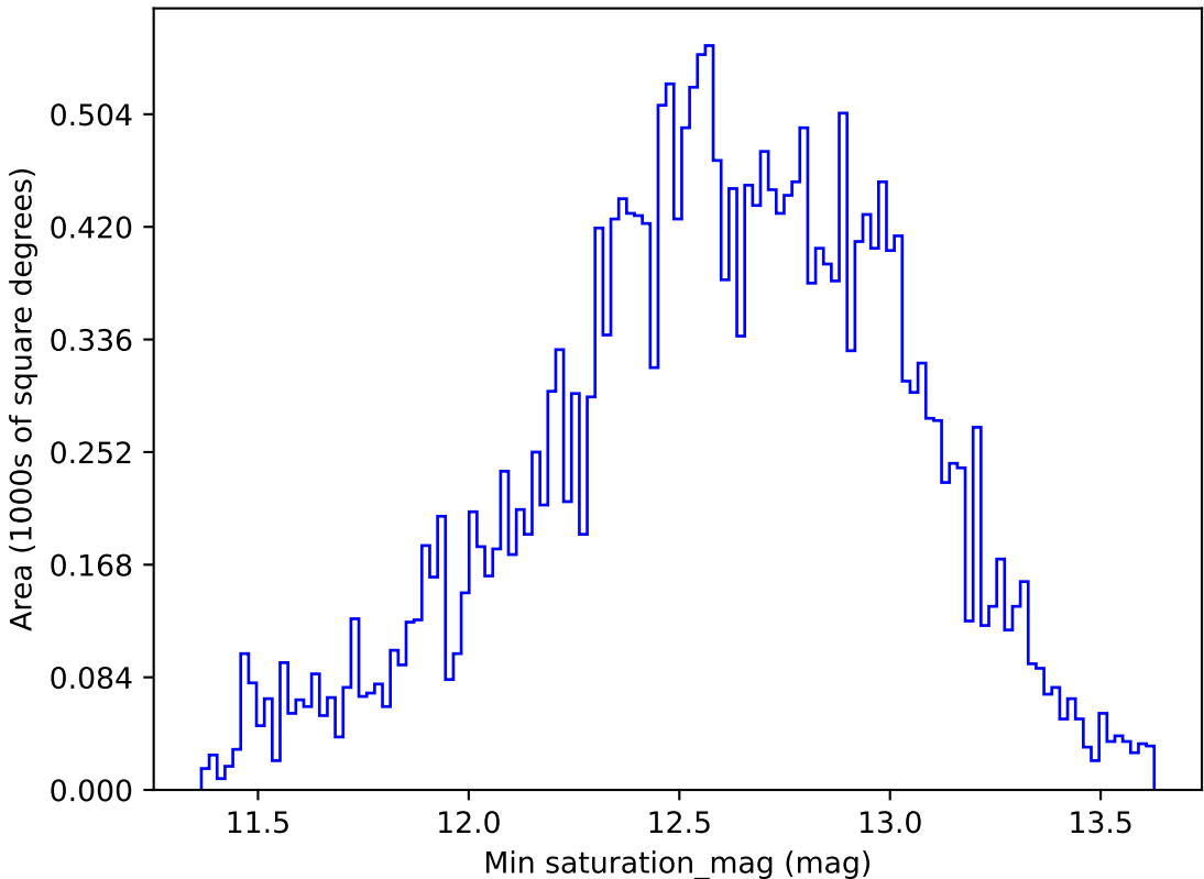
ddf_loaded_half_fl2_v3.4_10yrs All sky r band: Min saturation_mag
