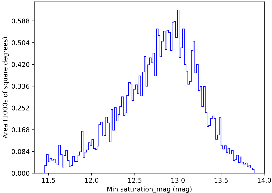
ddf_loaded_half_fl2_v3.4_10yrs All sky g band: Min saturation_mag
